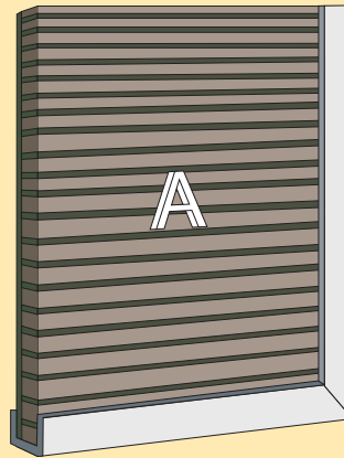
Style A Open face, no glass. 3/4" deep x 3/4" face.
