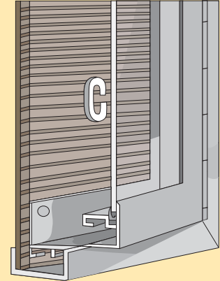
Style C Acrylic (1/8") door, continuous piano hinge, cylinder lock and key. 1 3/4" deep x 1 3/4" face.
